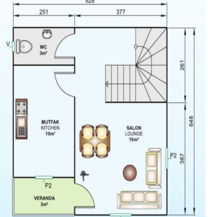
37 m 2 + 3 m 2 = 40 m 2 Zemin Kat Planı / Ground Floor Plan
